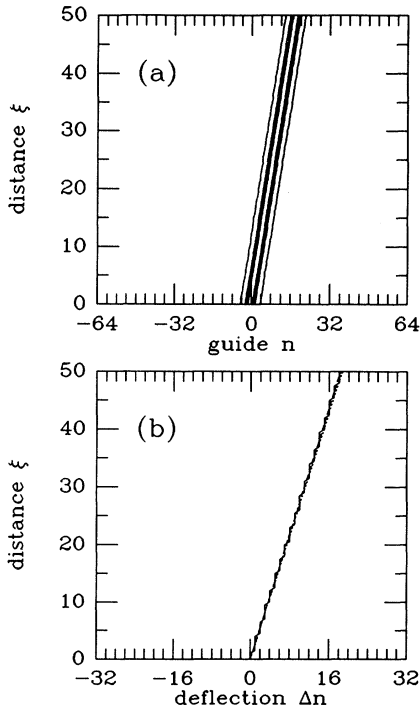
FIG. 12. Comparison between numerical and approximate analytical prediction for the movement of the DST soliton center of mass: (a) contour plot of soliton intensity for a weakly confined beam ( \mathcal{D}_{\text{SC}} = 0.43 ) and k = 0.2 ; (b) exact (solid line) and approximate (dots) trajectory for the beam center of mass.
