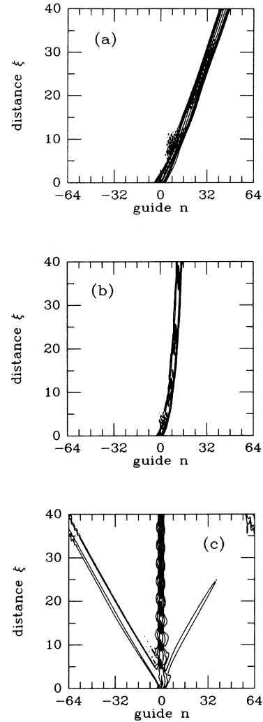
FIG. 21. Self-trapping of ALDNLs solitons. Contour plot of the beam intensity for k = 1 and different confinement parameters: (a) \mu = 0.5 ; (b) \mu = 0.75 ; (c) \mu = 1 .
