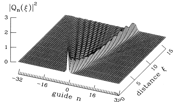
FIG. 8. Moving DST soliton with initial spatial frequency k = \pi/2 and \mathcal{D}_{\text{SC}} = 0.85 .
