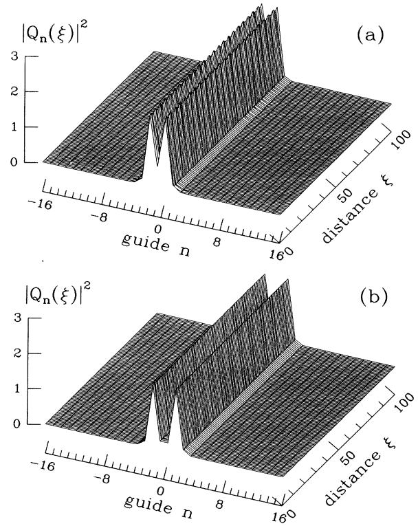
FIG. 3. Weak interactions of two well-confined DST solitons ( \mathcal{D}_{SC} = 0.85 ). Here \Delta = 2 (a) and \Delta = 3 (b).
